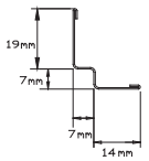
Shadow Molding 阶梯型边龙骨
